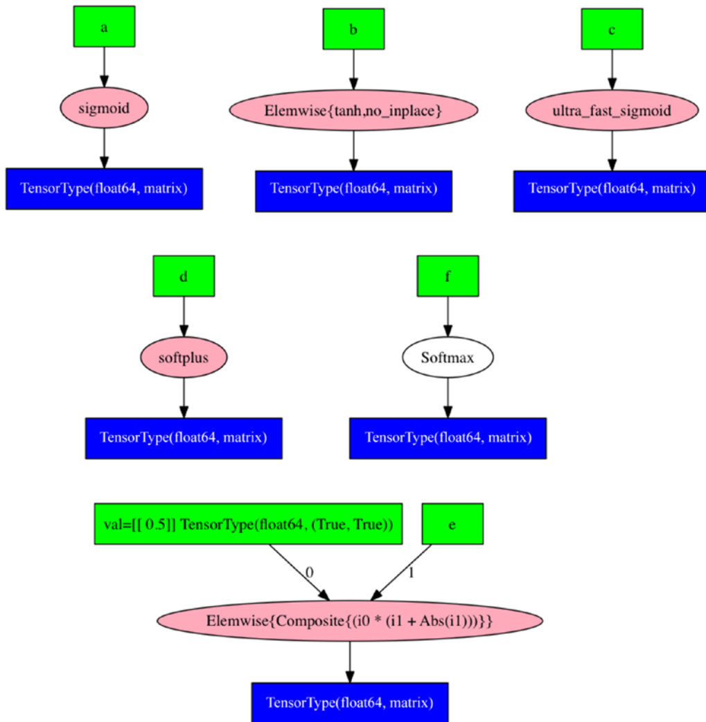
Figure 4-4. Activation Functions
