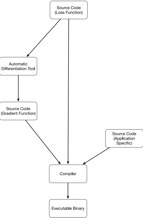
Figure 9-8. Source Code Transformation
