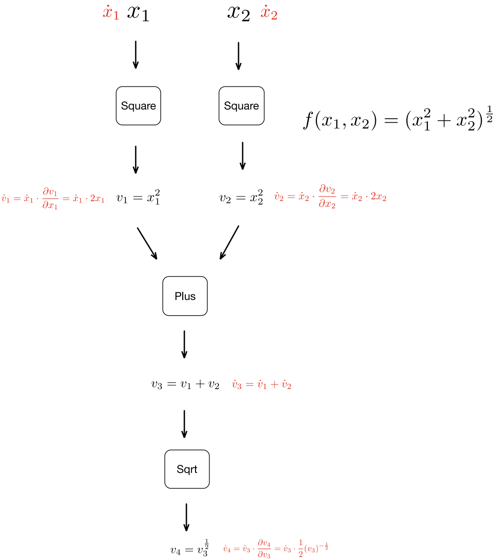
Figure 9-2. Associating every intermediate variable with a derivative in forward mode automatic differentiation
