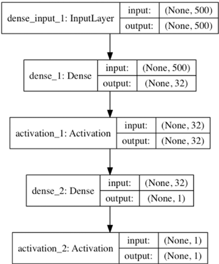
Figure 7-4. Regression
