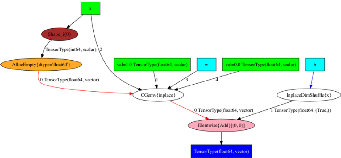
Figure 4-11. Linear Regression
