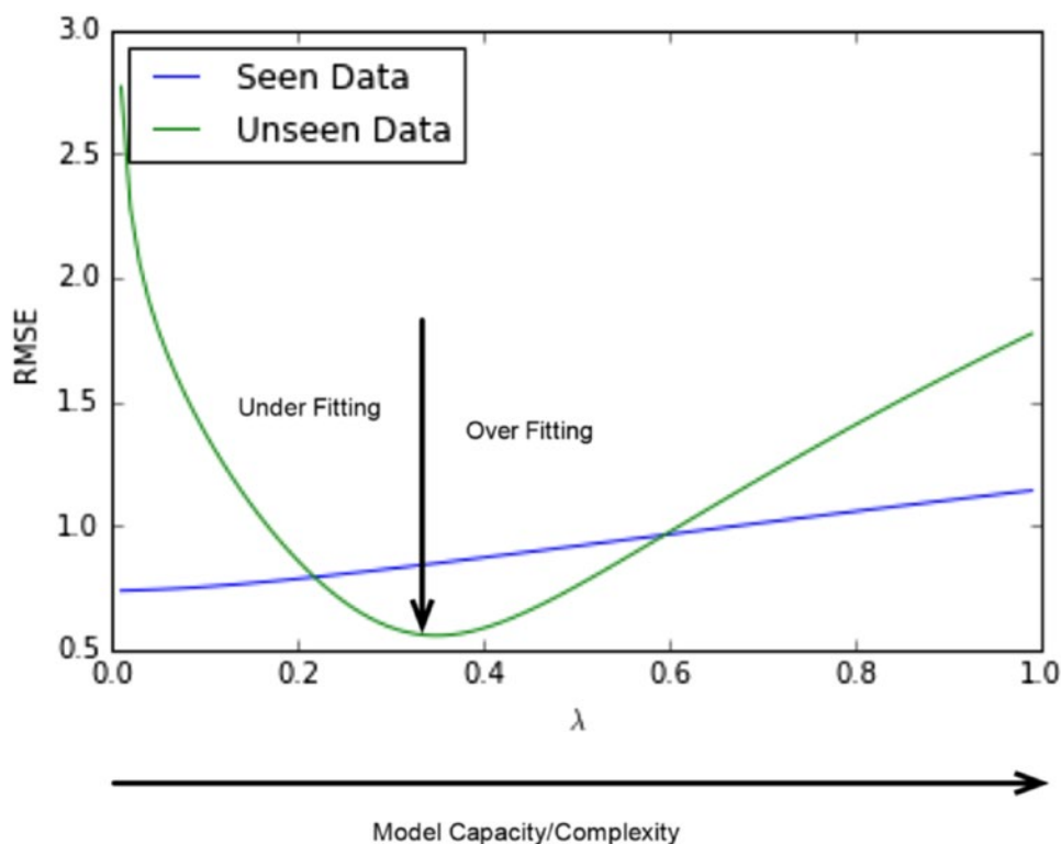
Figure 2-5. Regularization
